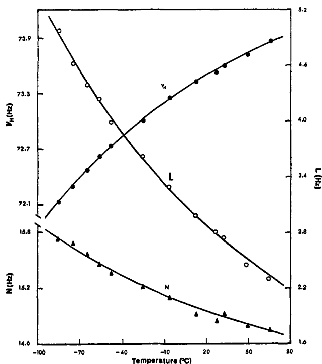
Figure 2. Observed temperature dependence of N (▲), L (○), and \nu_H (●) in neat 1. The solid lines are the calculated parameter temperature dependences for solution 4 ( \Delta S = 1.376 eu) in Table I.
